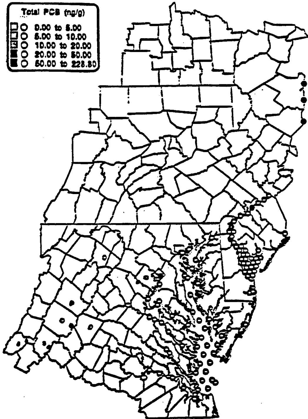
Figure 9. Total polychlorinated biphenyls (PCBs) per gram sediment reported for Chesapeake Bay, Delaware Bay and DE & MD coastal bays by E-map data (provided by NOAA/ORCA/SEA).
