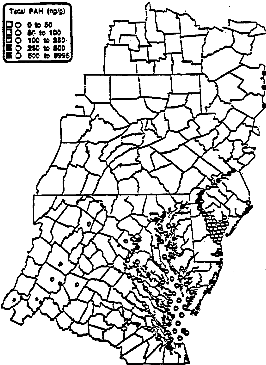
Figure 8. Total polycyclic aromatic hydrocarbons (PAHs) reported per gram sediment for Chesapeake Bay, Delaware Bay and DE & MD coastal bays by E-map data (provided by NOAA/ORCA/SEA).
