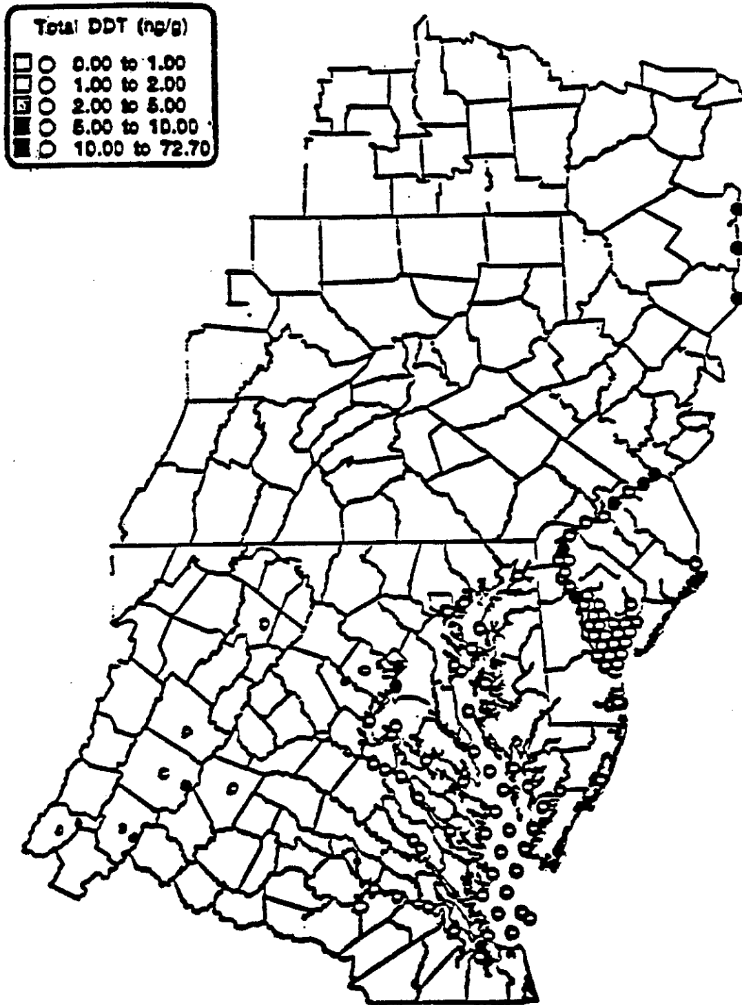
Figure 10. Total DDT (dichloro-diphenyl-trichloroethane) and its metabolites per gram sediment for Chesapeake Bay, Delaware Bay and DE & MD coastal bays by E-map data (provided by NOAA/ORCA/SEA).
