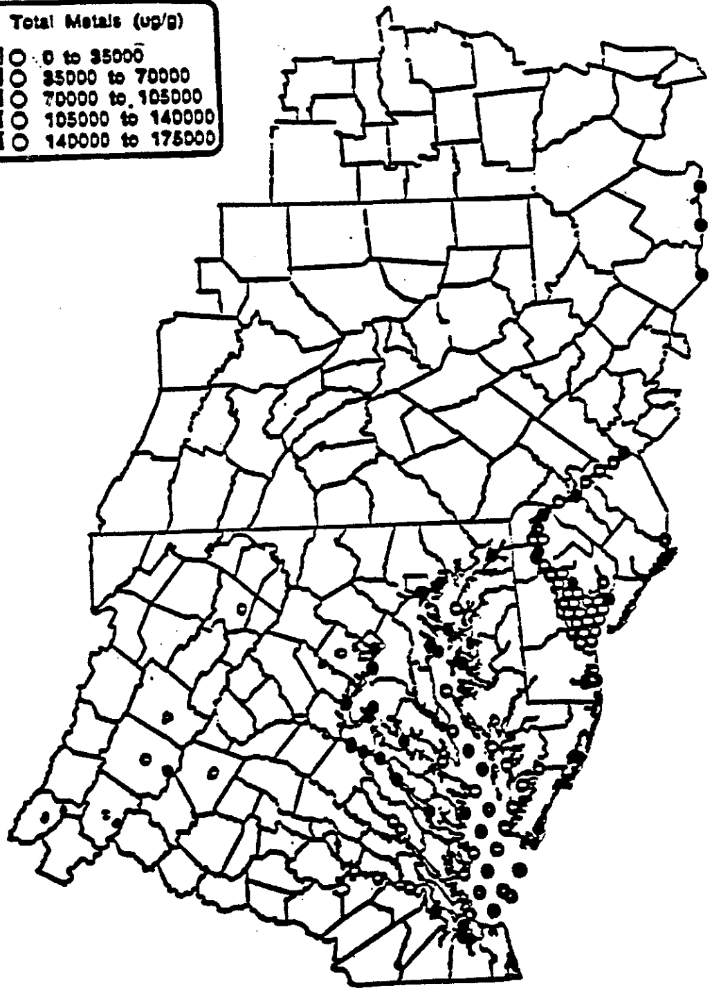
Figure 7. Total metals reported per gram sediment for Chesapeake Bay, Delaware Bay and MD coastal bays by E-Map data (provided by NOAA/ORCA/SEA).
