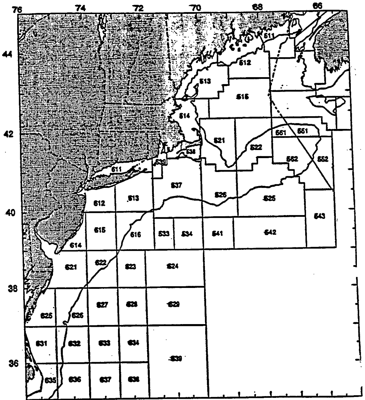
Figure 15. Statistical areas used for catch monitoring in offshore fisheries in the northeast United States
