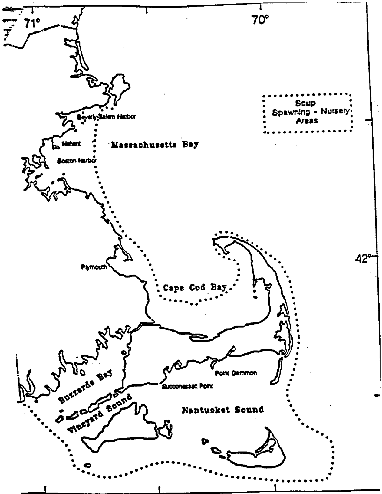
Figure 5. Scup habitat in Massachusetts waters.
