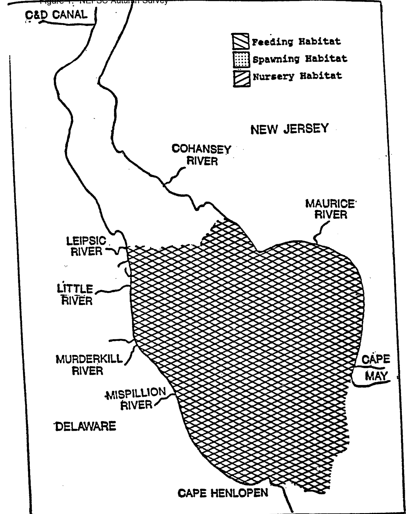
Figure 2. Scup nursery/feeding habitat distribution in Delaware Bay.
