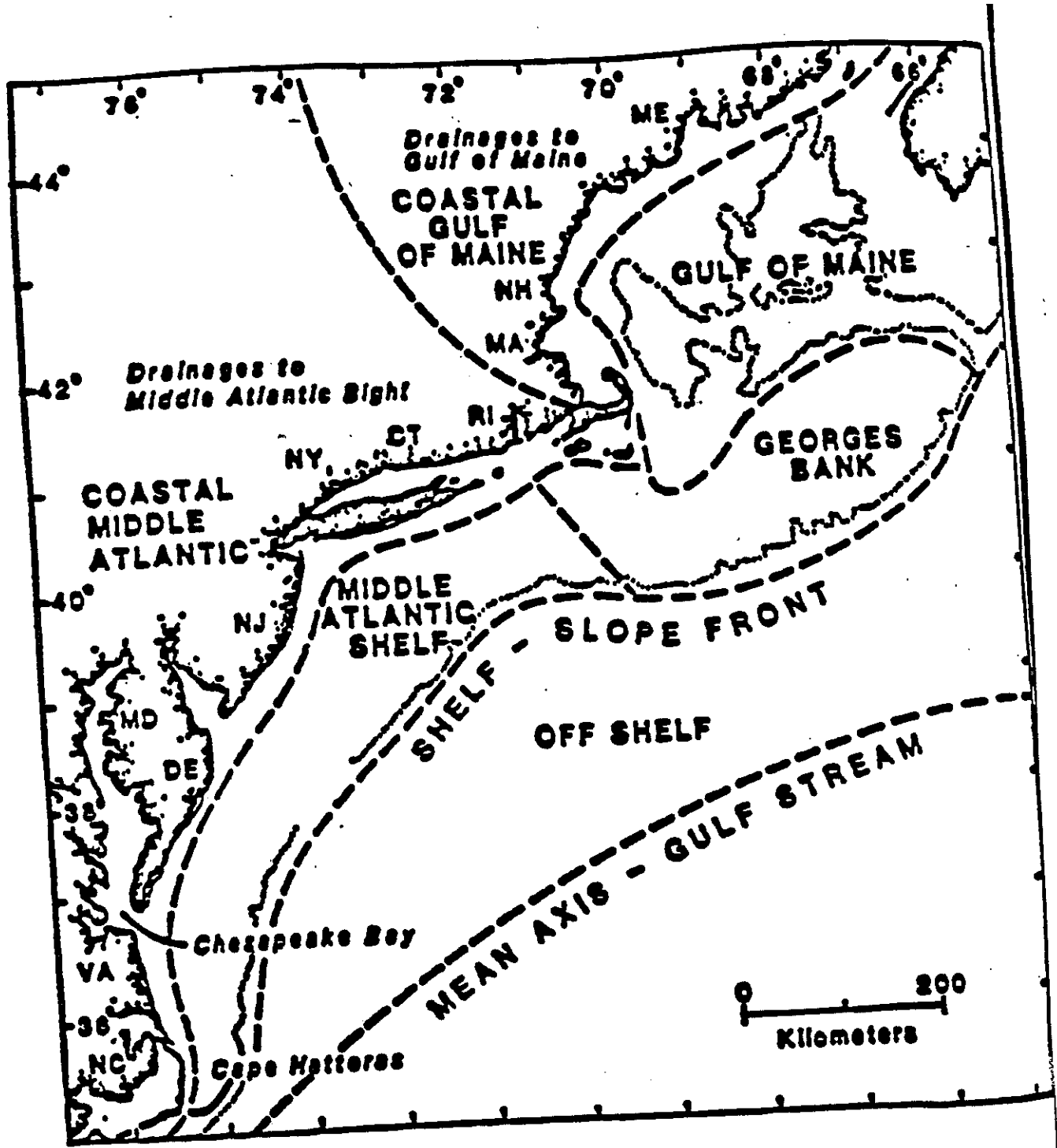
Figure 11. Northeast Regional Action Plan (RAP) Water Management Units.
