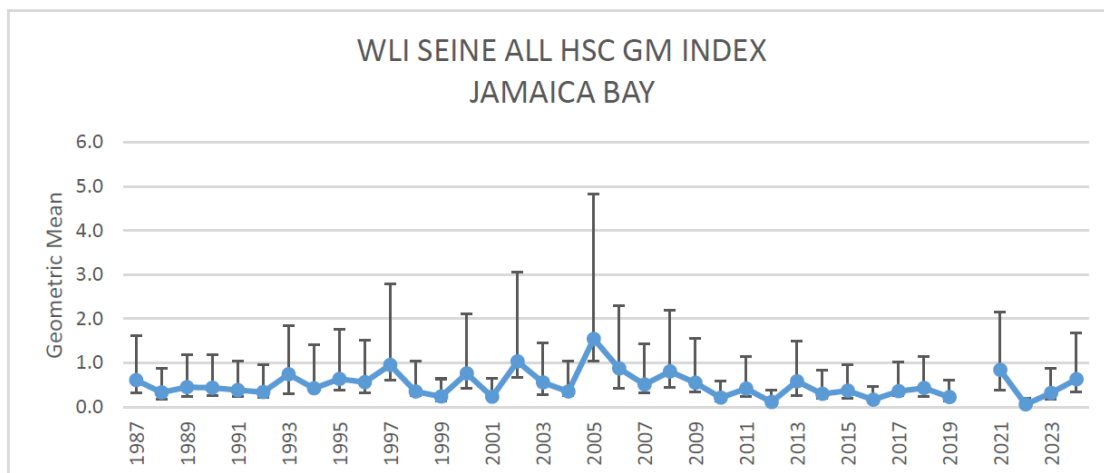
Figure 6. NYSDEC WLI Jamaica Bay Beach Seine Survey All Horseshoe Crab GM Index, 1987-2024. *Due to the COVID-19 pandemic, in 2020 sampling did not begin until July.
