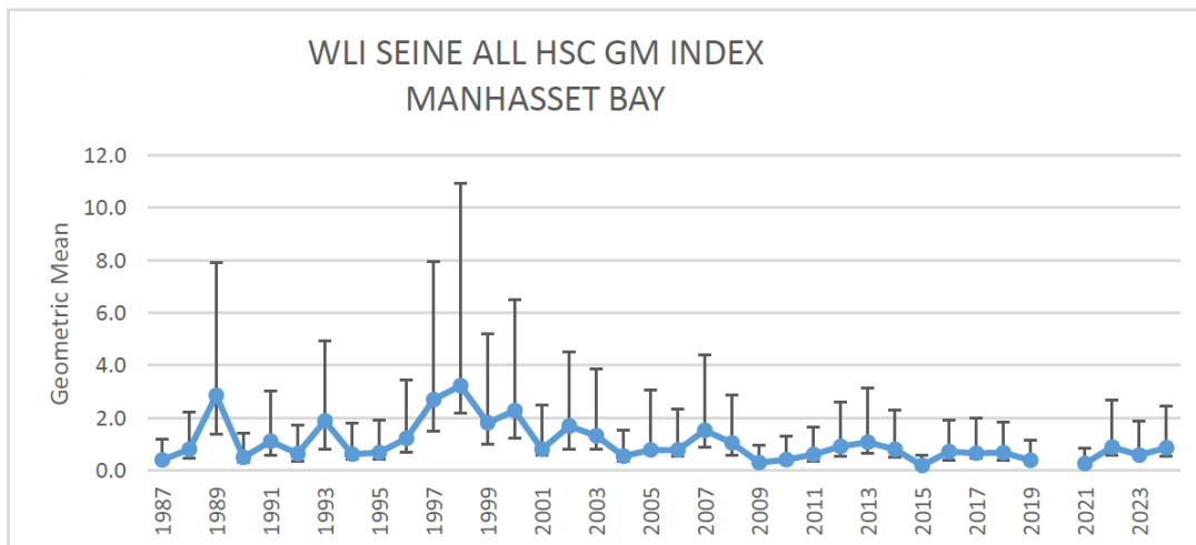
Figure 8. Manhasset Bay Seine Survey All Horseshoe Crab GM Index, 1987-2024. *Due to the COVID-19 pandemic, in 2020 sampling did not begin until July.
