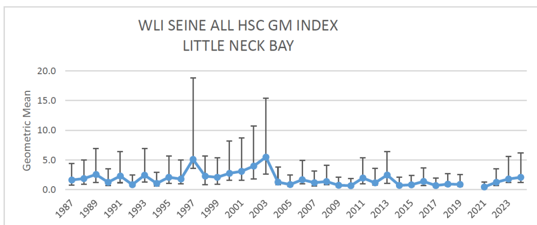
Figure 7. Little Neck Bay Seine Survey All Horseshoe Crab GM Index, 1987-2024. *Due to the COVID-19 pandemic, in 2020 sampling did not begin until July.
