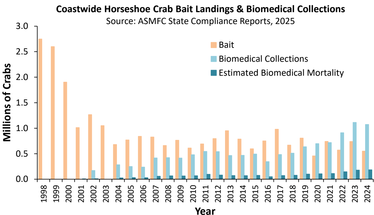
Figure 2. Horseshoe crab bait harvest, biomedical collections, and biomedical mortality, 1998-2024.
