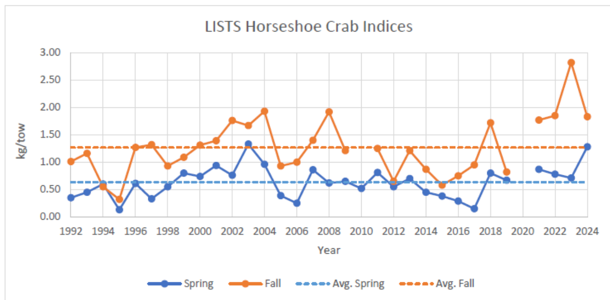
Figure 4. LISTS Horseshoe Crab Indices, 1992-2024.
