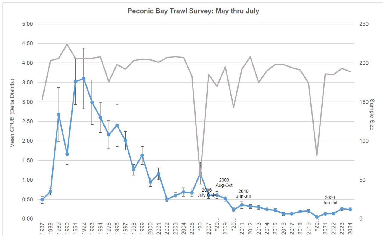
Figure 5. Peconic Bay Trawl Survey: May through July, 1987-2024. (Gray line=sample size, blue line=mean CPUE).
