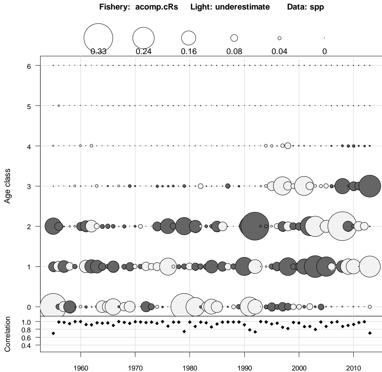
Figure 10. Relative (upper panel) and absolute (lower panel) bubble plots of the residuals of the predicted catch-at-age for Atlantic menhaden from 1955-2013 from Virginia Eastern Shore and south by the commercial reduction fishery. The error degrees in the upper panel represents a composite fit by year across ages, while in the lower plot contains correlations between years.
