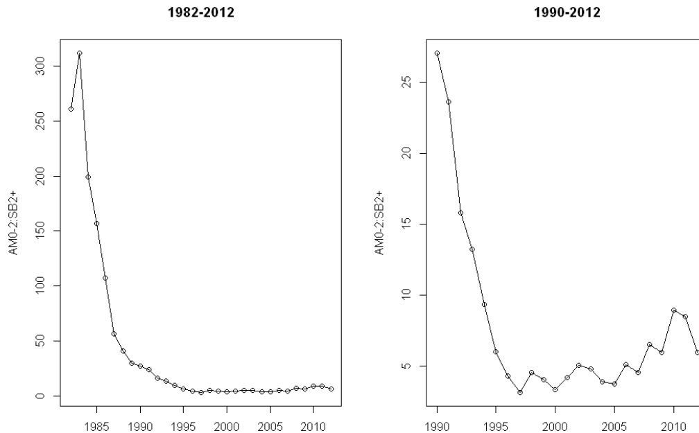
Figure 6. Prey: predator ratios for ages 0-2 menhaden and ages 2+ striped bass. To help illustrate trends in the ratio towards the end of the time series the plot on the right excludes ratios from 1982-1989. The figures are the same otherwise.
