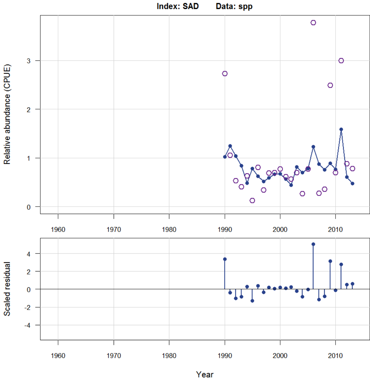
Figure 7.1.15. The observed and predicted SAD index for 1990-2013 comprised of two state trawl surveys in the southern region.
