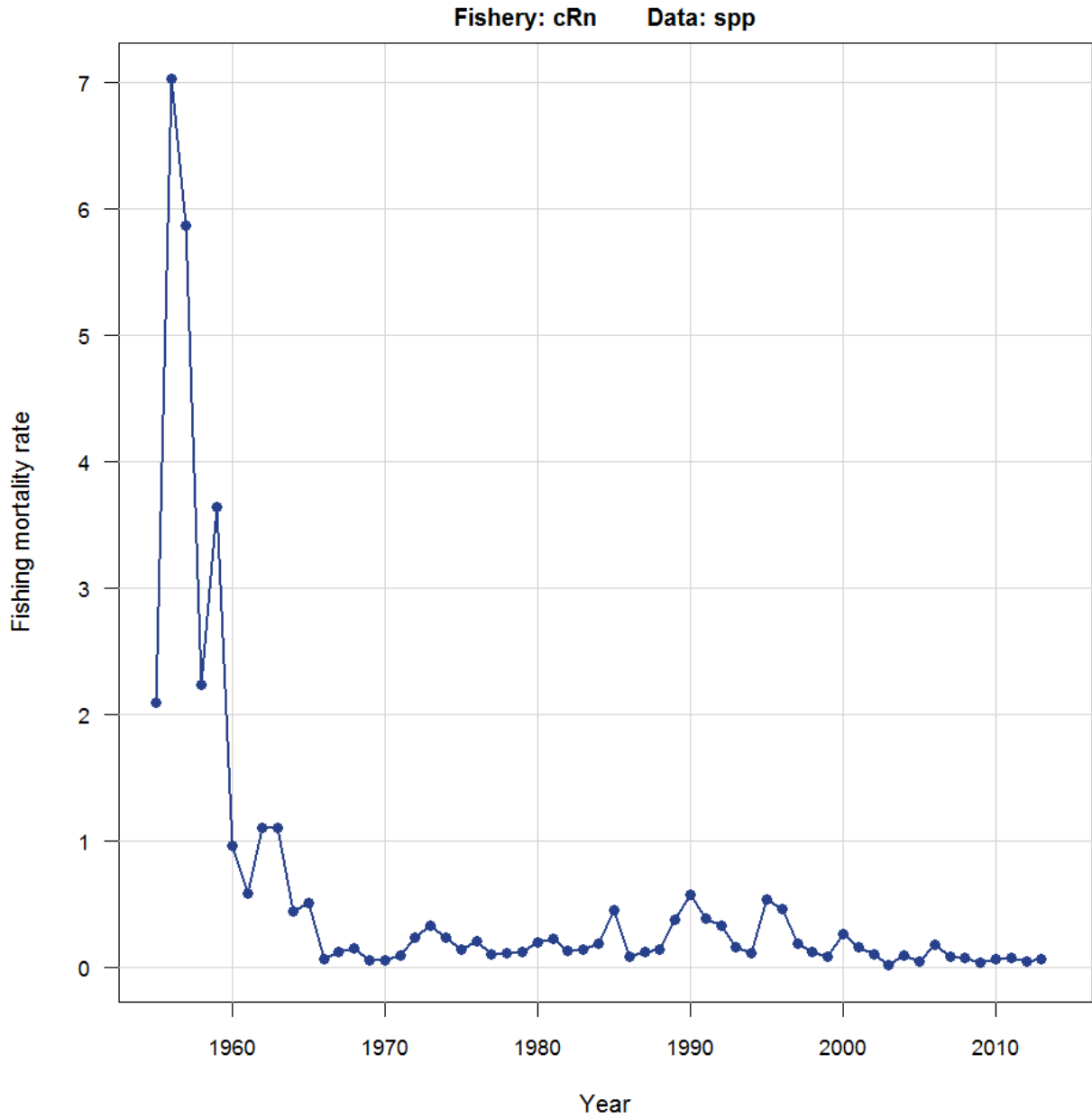
Figure 30. Fishing mortality rate for the northern commercial reduction fishery from 1955-2013.
