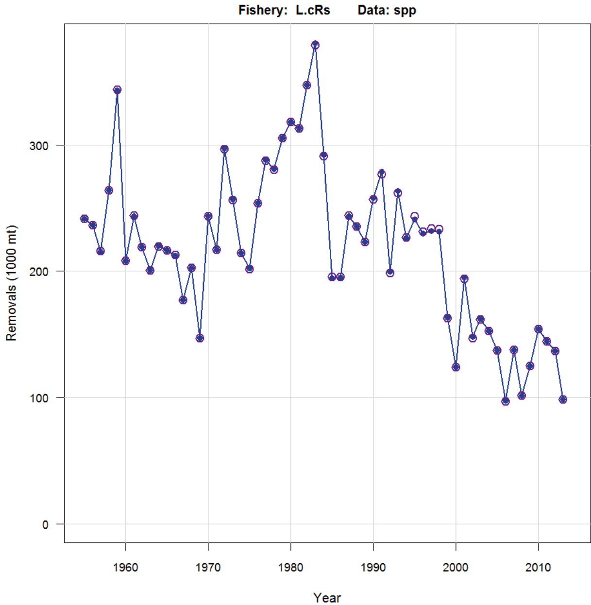
Figure 2. Observed and predicted removals of Atlantic menhaden from 1955-2013 from Virginia Eastern Shore and south by the commercial reduction fishery.
