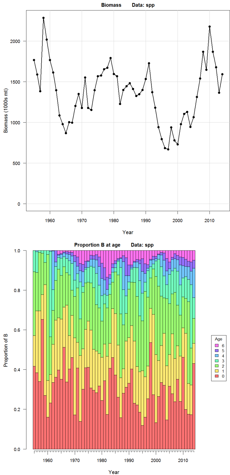
Figure 7.2.3.3. Biomass (upper panel) and biomass at age (lower panel) over time as predicted from the base run of the BAM for Atlantic menhaden.
