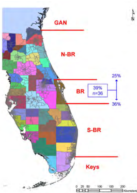
Figure 2.2. Movement of tagged cobia from Brevard County, FL (BR) to the north and south.
