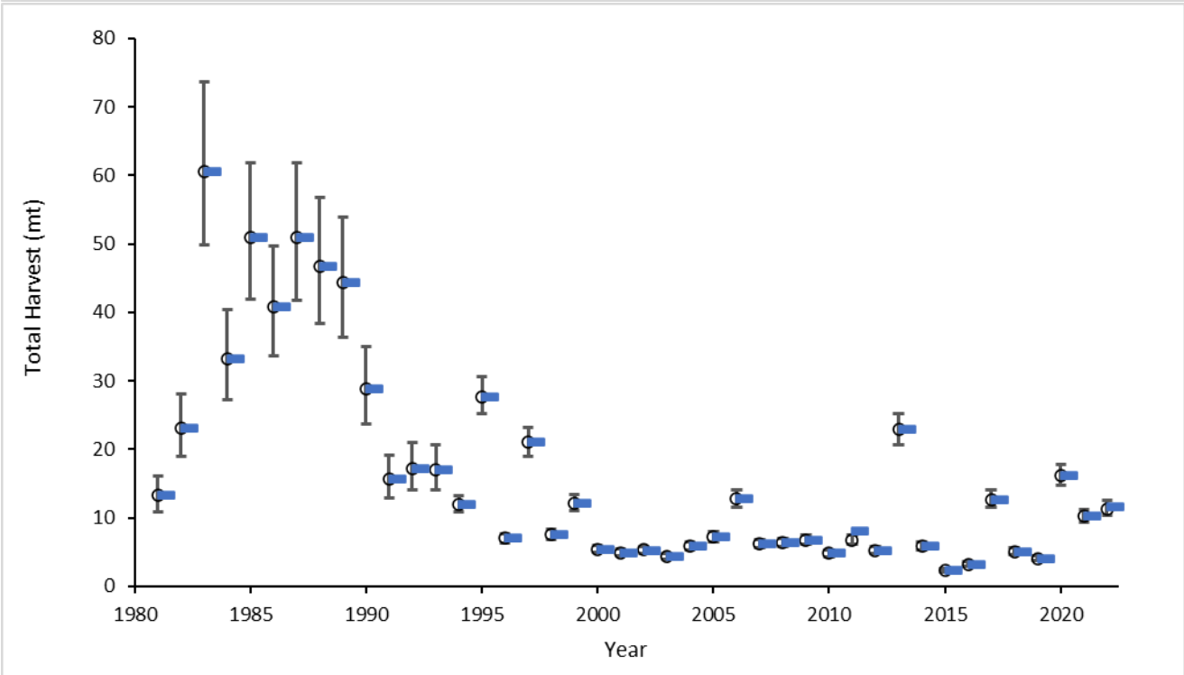
Figure 128. Observed and estimated catches for the North_Commercial_Other fleet for the northern stock SS estimated selectivity model (top) and hybrid selectivity model (bottom).
