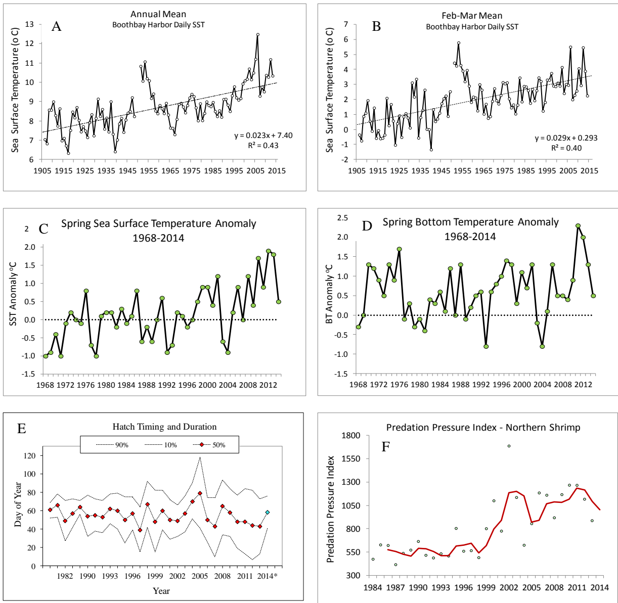
Figure 17: Annual temperature, predation pressure, and hatch timing and duration for northern shrimp in the Gulf of Maine. (A) Average annual sea surface temperature (SST) and (B) average SST during February-March at Boothbay Harbor, Maine, 1906-2014. (C) Spring sea surface temperature anomaly in shrimp offshore habitat areas from NEFSC trawl surveys, 1968-2014. (D) Spring bottom temperature anomaly in shrimp offshore habitat areas from NEFSC trawl surveys, 1968-2014. (E) Estimated hatch timing (10%=start, 50%=midpoint, 90%=completion) for northern shrimp in the Gulf of Maine, 1980-1983 and 1989-2014 (no data 1984-1988). (F) Predation pressure index for northern shrimp in the Gulf of Maine, 1984-2013.
