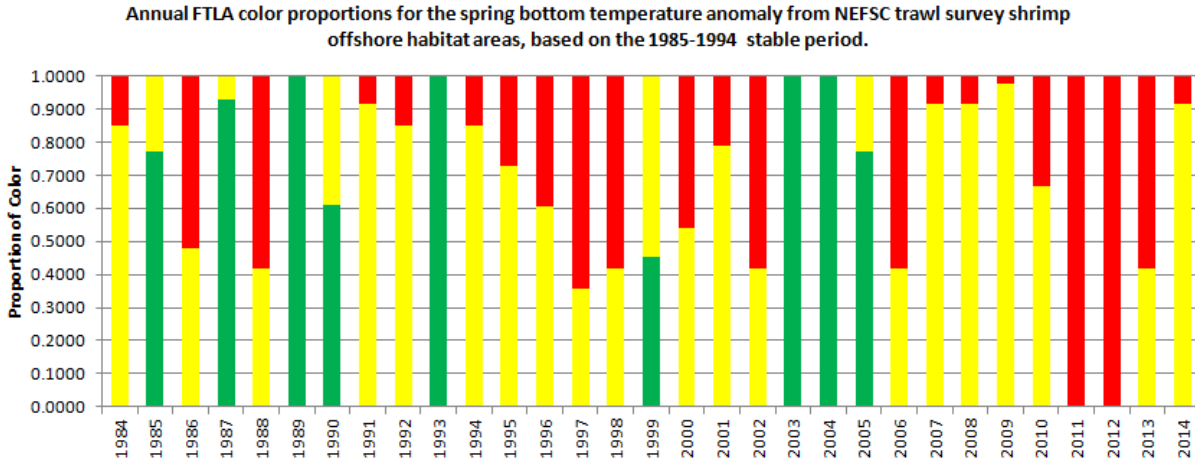
Figure 26: Spring bottom temperature anomaly from the NEFCS trawl survey in shrimp offshore habitat areas from 1984-2014. Top: annual index relative to the stable period mean (SPM) (dashed line) and to the 80th percentile of the time series from 1984-2014 (dotted line). Green dots are values \leq SPM; red dots are values \geq the 80th percentile of the time series; yellow dots are values between the SPM and the 80th percentile. Bottom: annual color proportions indicate proximity to the SPM (red = unfavorable; green = favorable).
