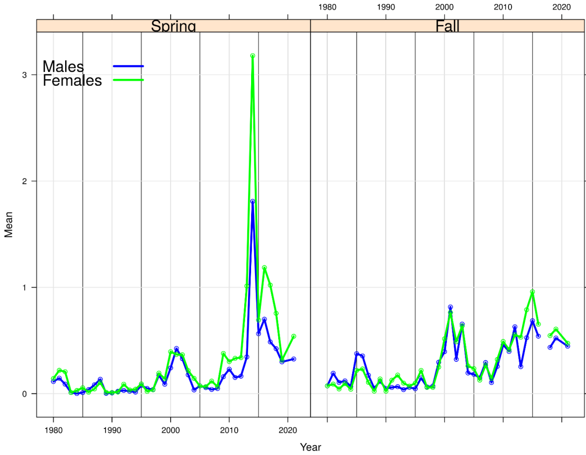
Figure 11. NMFS Jonah Crab index (mean number per tow) from the bottom trawl survey for the NEFSC Survey Area, through fall 2021. There was no survey conducted in 2020 due to the COVID-19 pandemic.
