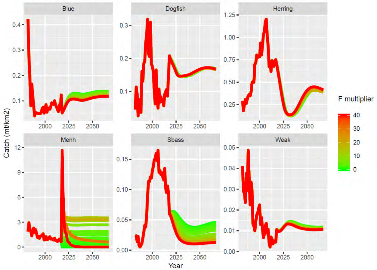
Catch predictions under diff. Menh F rates (w/ ERP spp at F_{tar} ) – Sim2
