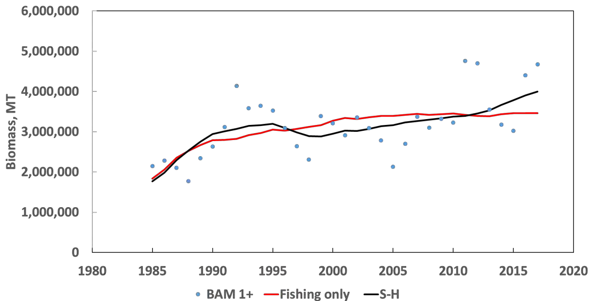
Figure 11. Time-series (1985-2017) of ages 1+ Atlantic menhaden biomass estimated by BAM, and time-series of ages 1+ Atlantic menhaden biomass estimated by a fishing only biomass dynamic model and a Steele-Henderson model (fishing and Striped Bass predation) fit to BAM biomass estimates.
