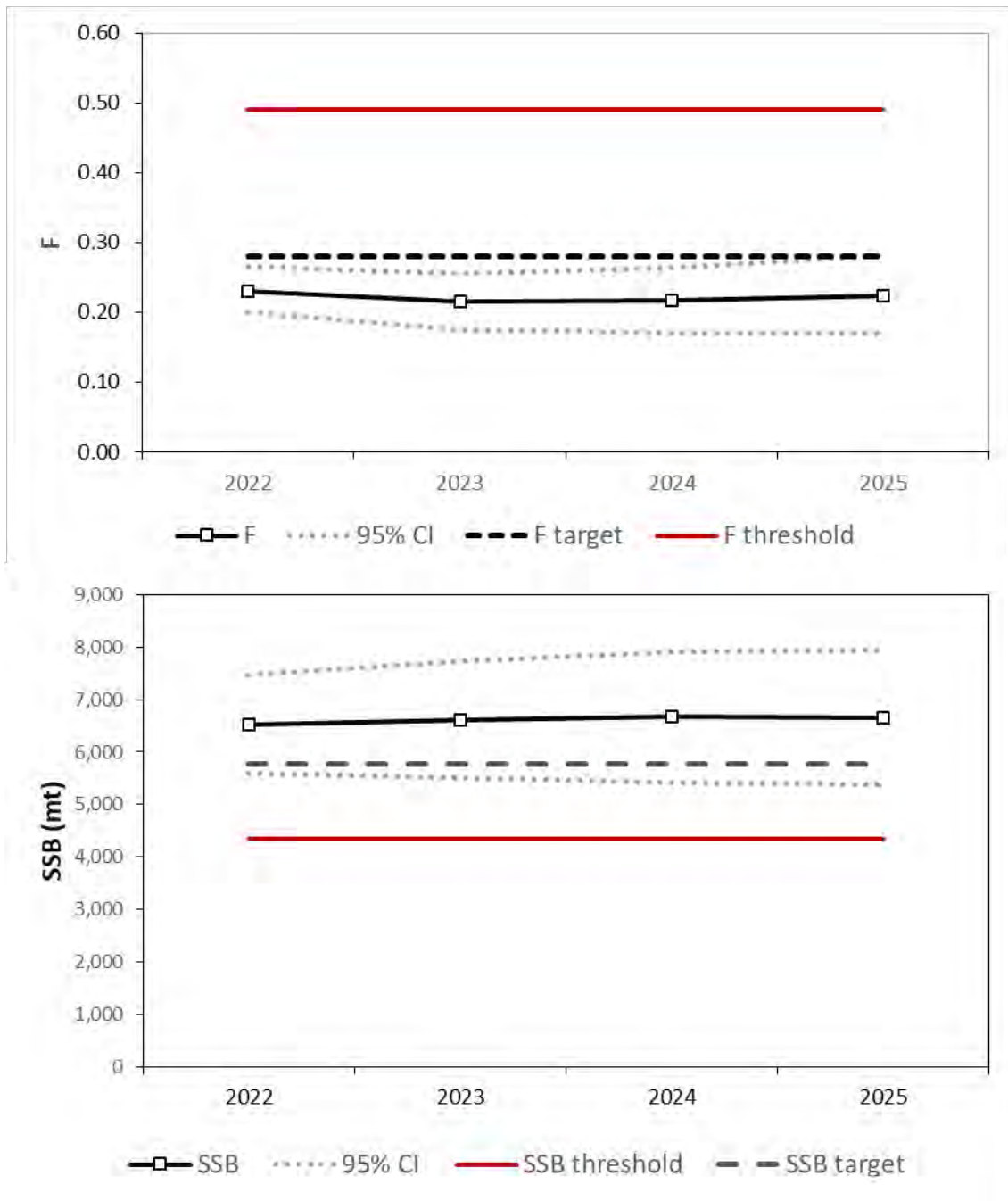
Figure 11. Status quo harvest projections for the MARI region showing the trajectory of annual F (top) and SSB (bottom) with their target and threshold reference points. Dotted grey lines indicate the 95% confidence intervals of the estimates.
