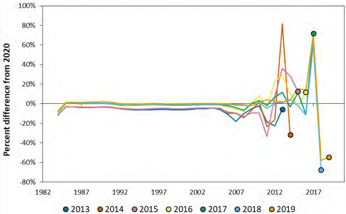
Figure 20. Retrospective analysis for annual recruitment from the LIS region in absolute numbers (top) and percent difference (bottom).
