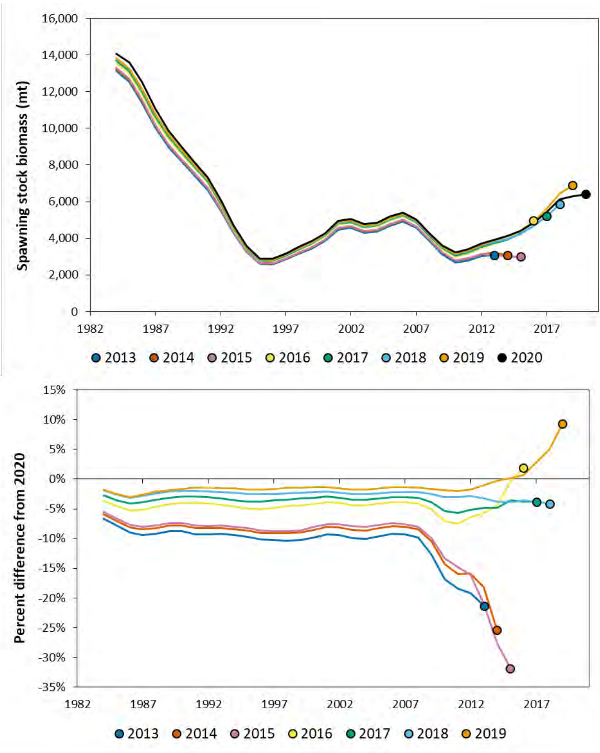
Figure 19. Retrospective analysis for annual SSB from the LIS region in absolute numbers (top) and percent difference (bottom).
