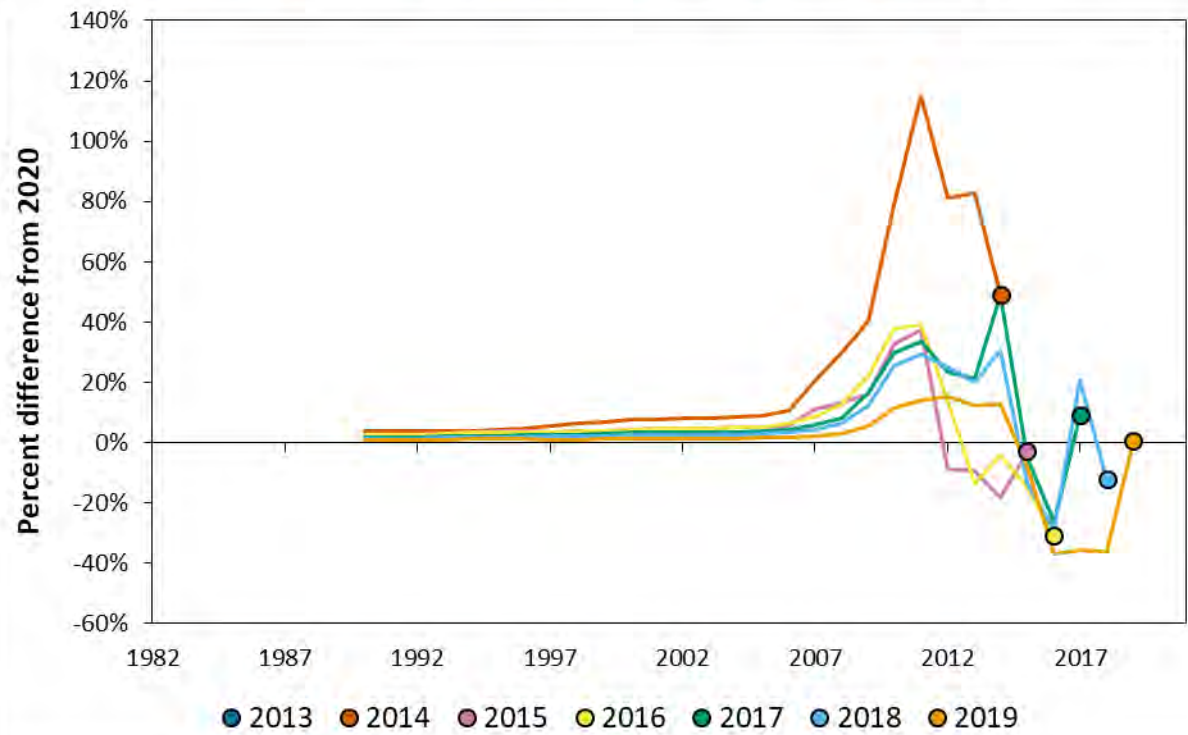
Figure 42. Retrospective analysis for recruitment in absolute numbers (top) and percent difference (bottom) for the DMV region.
