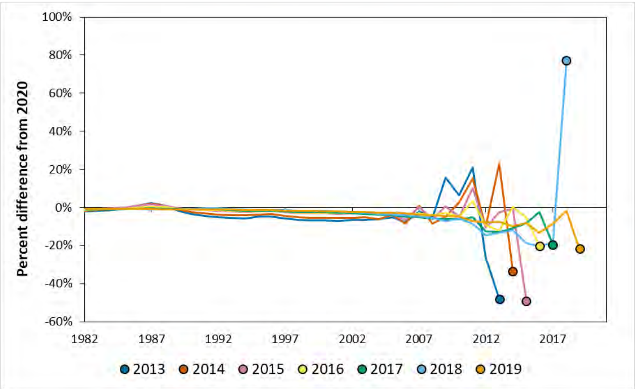
Figure 9. Retrospective analysis for recruitment for the MARI region in absolute numbers (top) and percent difference (bottom).
