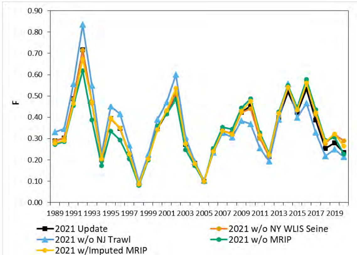
Figure A2.1. Annual F estimates from sensitivity runs without NY Seine index, without NJ Trawl index, without MRIP index, and with the MRIP index using imputed values.
