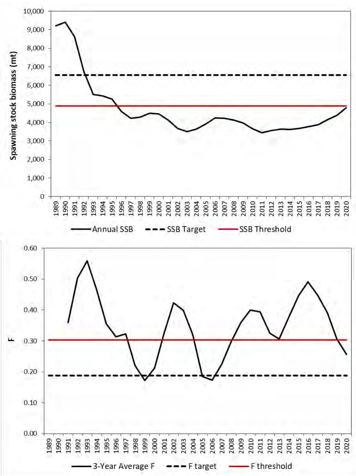
Figure 32. Annual SSB plotted with SSB target and threshold (top) and 3-year average F plotted with F target and threshold (bottom) for the NJ-NYB region.
