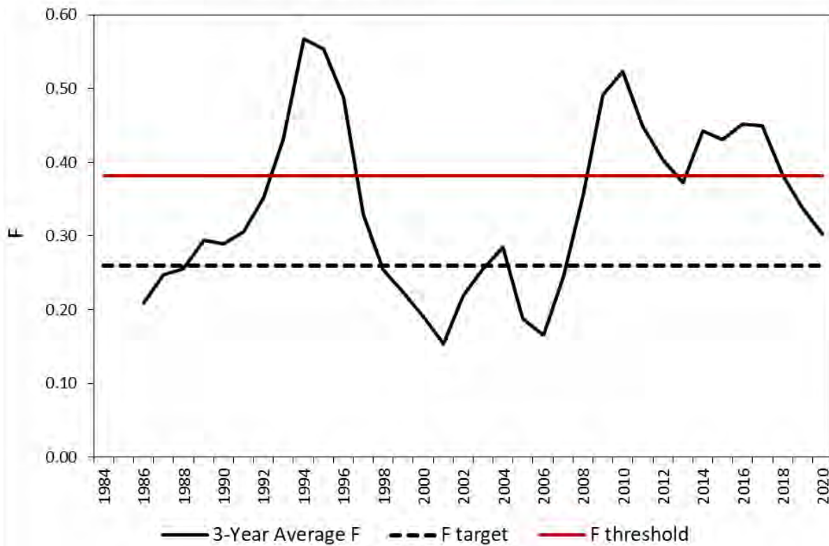
Figure 21. Annual SSB plotted with SSB target and threshold (top) and 3-year average F plotted with F target and threshold (bottom) for the LIS region.
