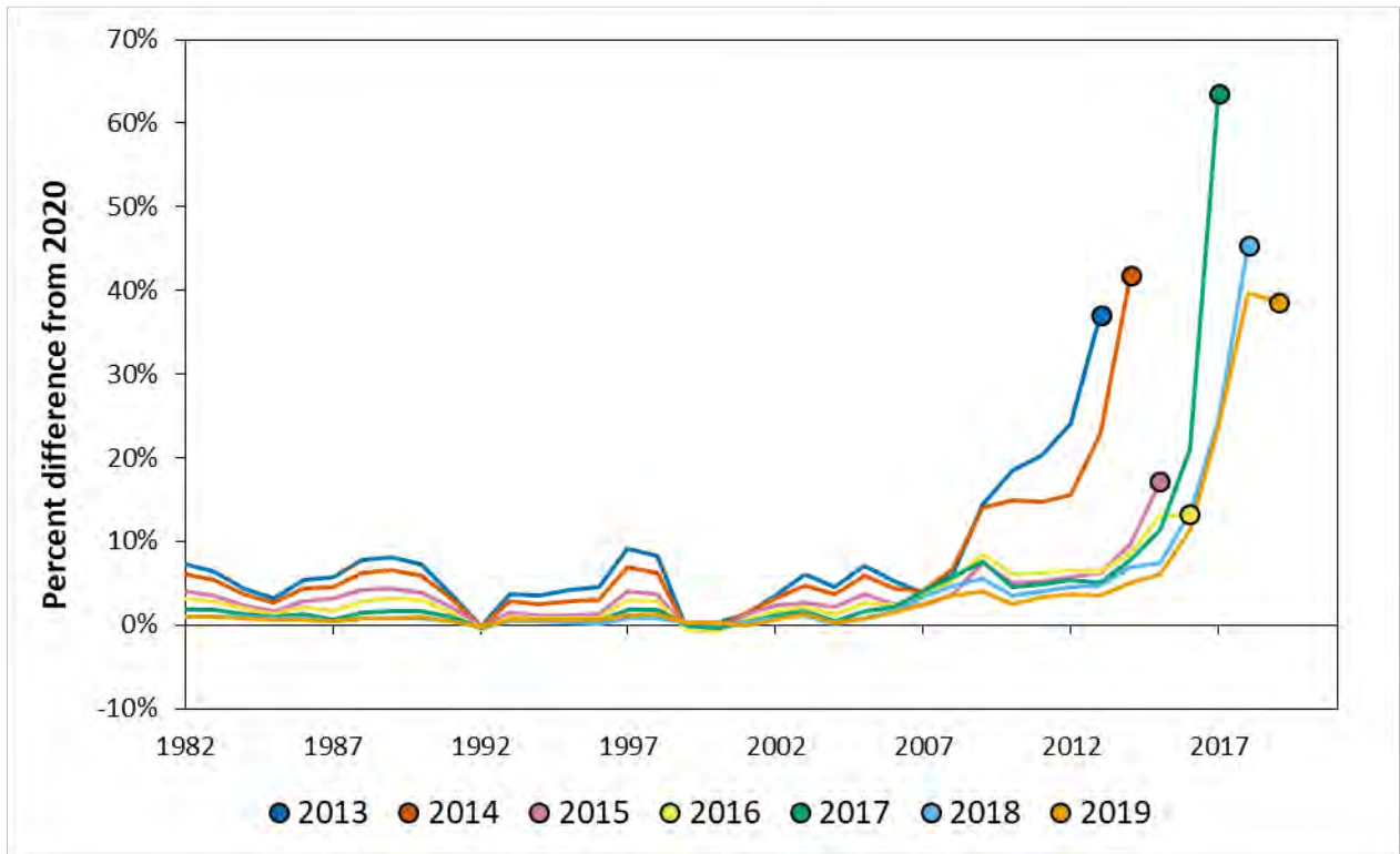
Figure 7. Retrospective analysis for annual F for the MARI region in absolute numbers (top) and percent difference (bottom).
