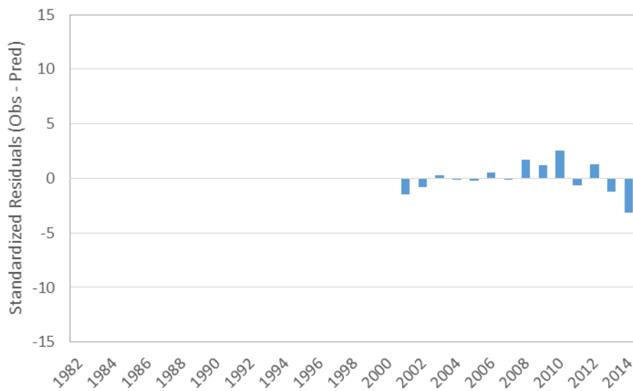
Figure 8.2.8. Observed and predicted values and standardized residuals from the North Carolina Pamlico Sound Independent Gillnet Survey from the ASAP model.
