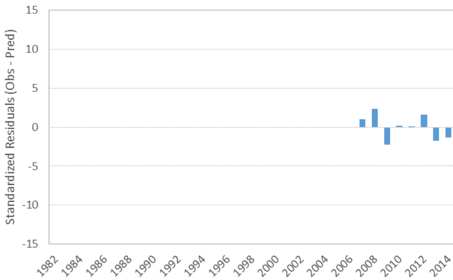
Figure 8.2.4. Observed and predicted values and standardized residuals for the NEAMAP survey from the ASAP model.
