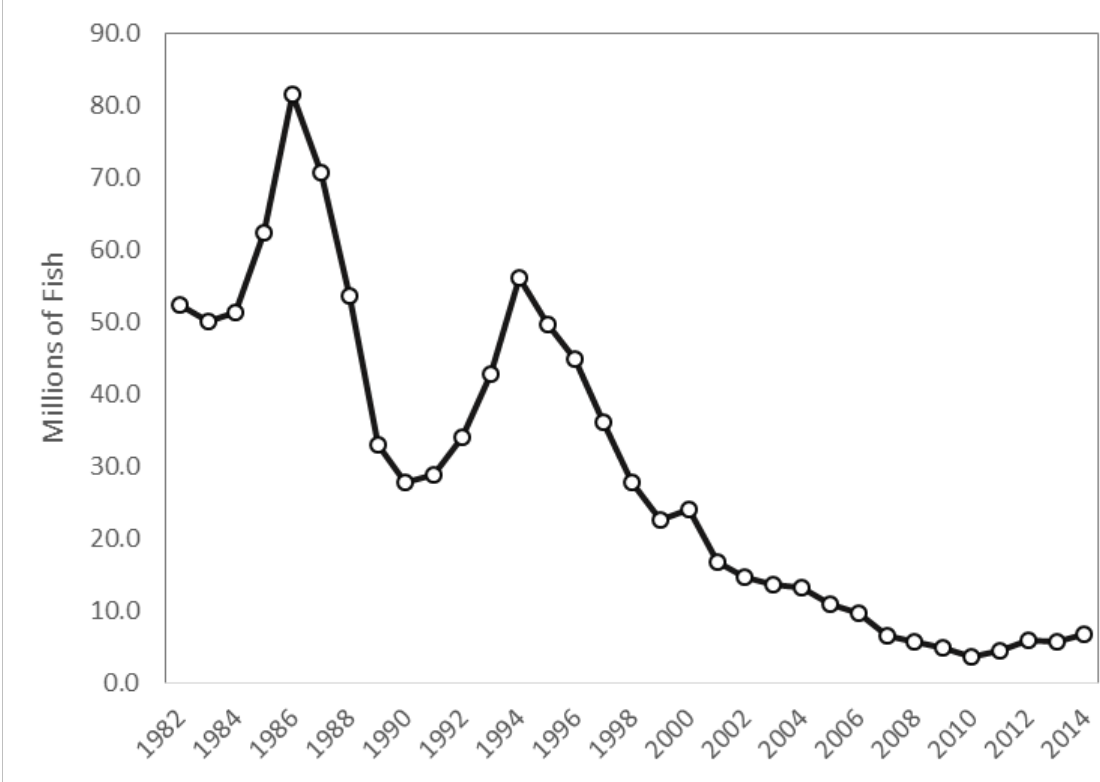
Figure 8.2.13. Total abundance estimated by the ASAP model.
