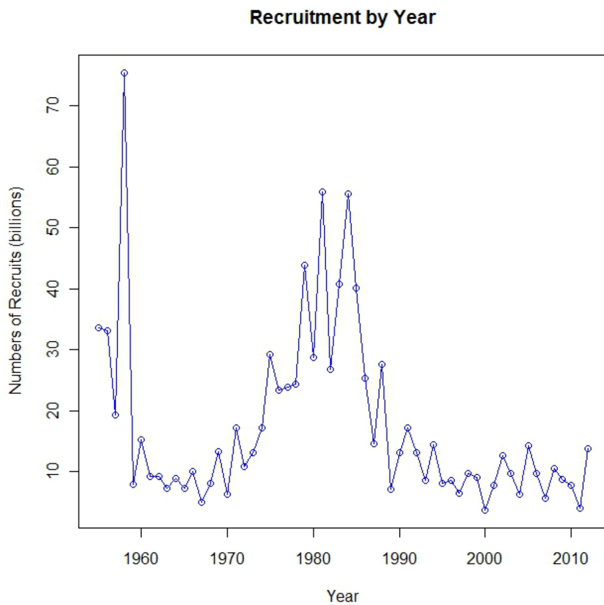
Figure 6. Estimated annual recruitment to age-0 (billions) from the base BAM model.
