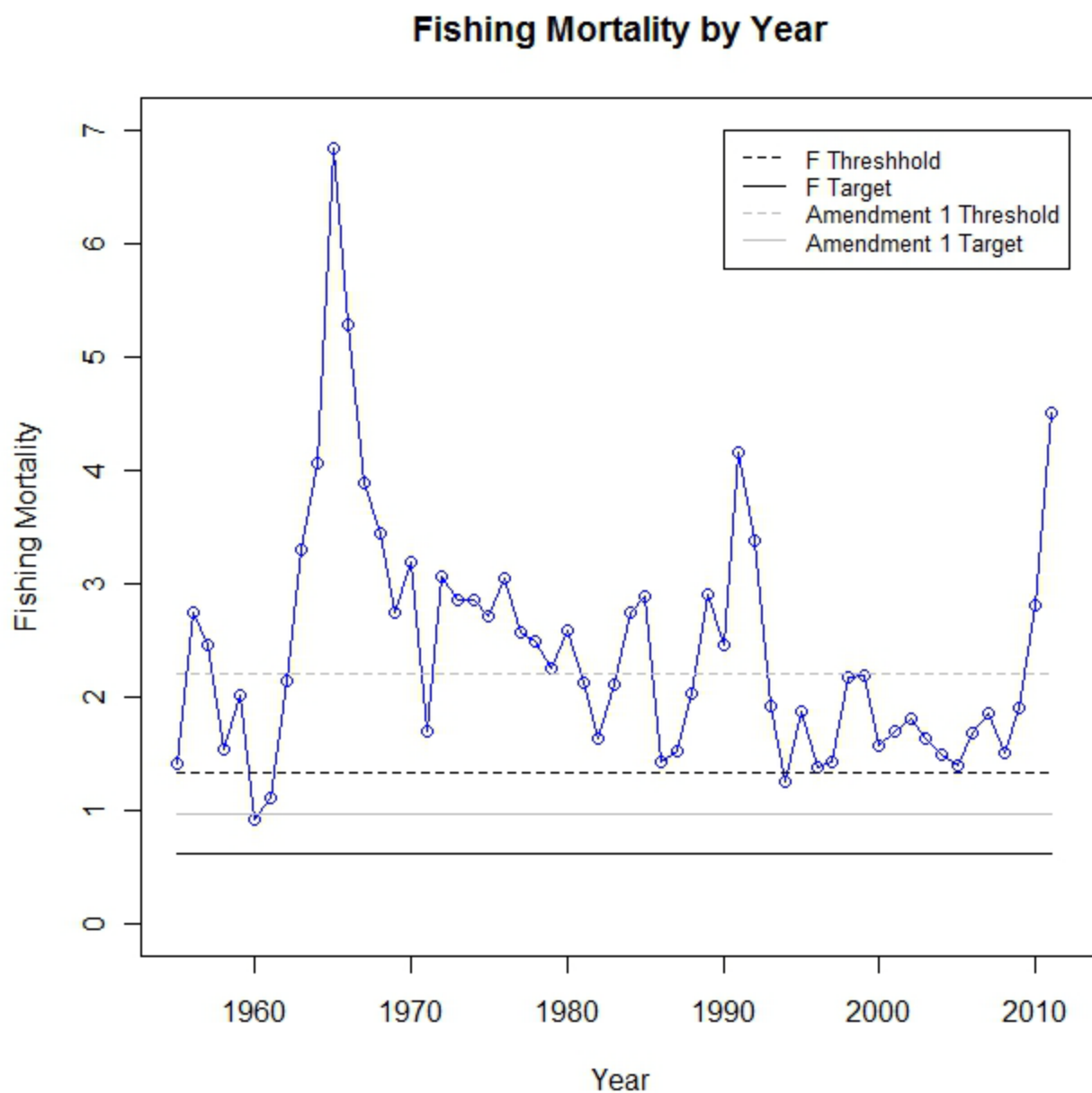
Figure 5. Estimated annual full fishing mortality rate from the base BAM model. Included are the F_{15\%MSP} threshold and F_{30\%MSP} target lines.
