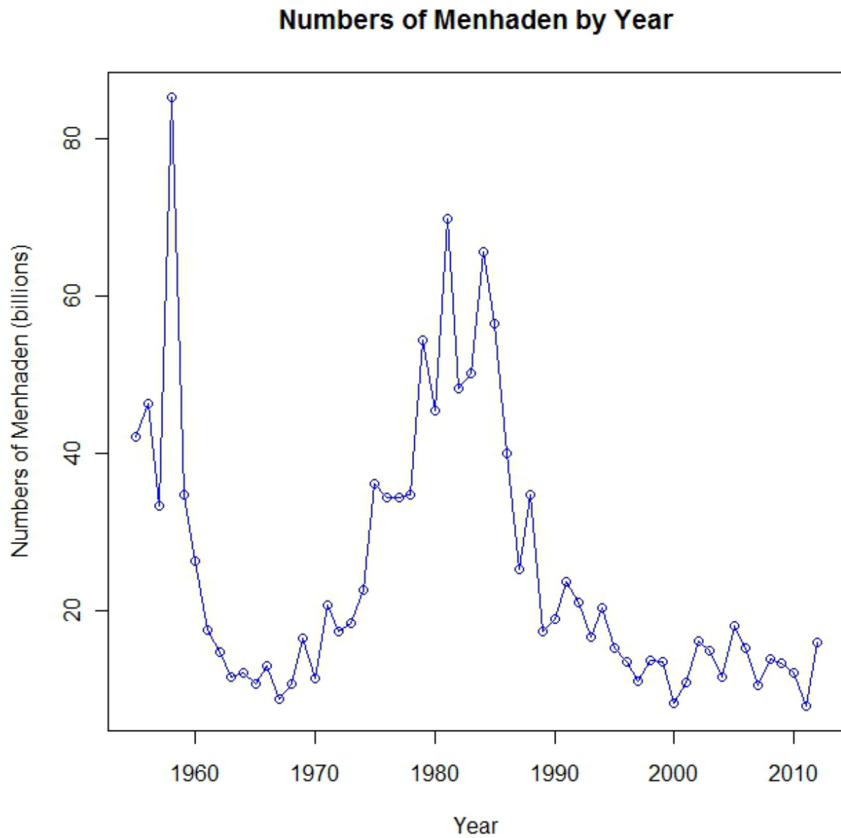
Figure 4. Estimated numbers at age of Atlantic menhaden (billions) at the start of the fishing year from the base BAM model.
