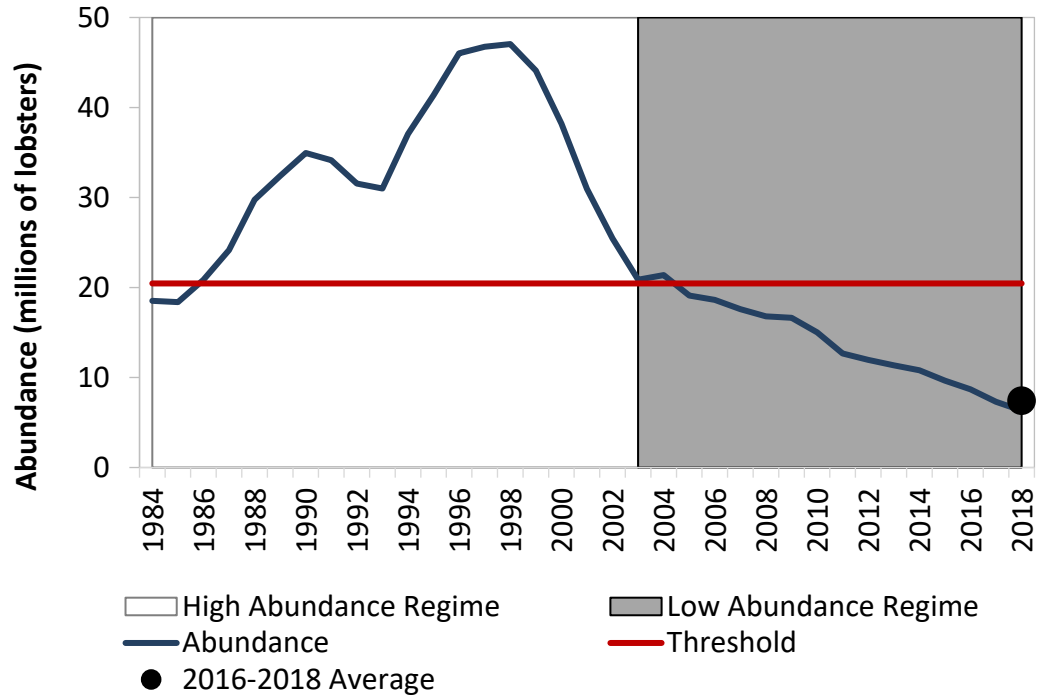
Figure 3. Abundance for SNE Relative to Reference Points
