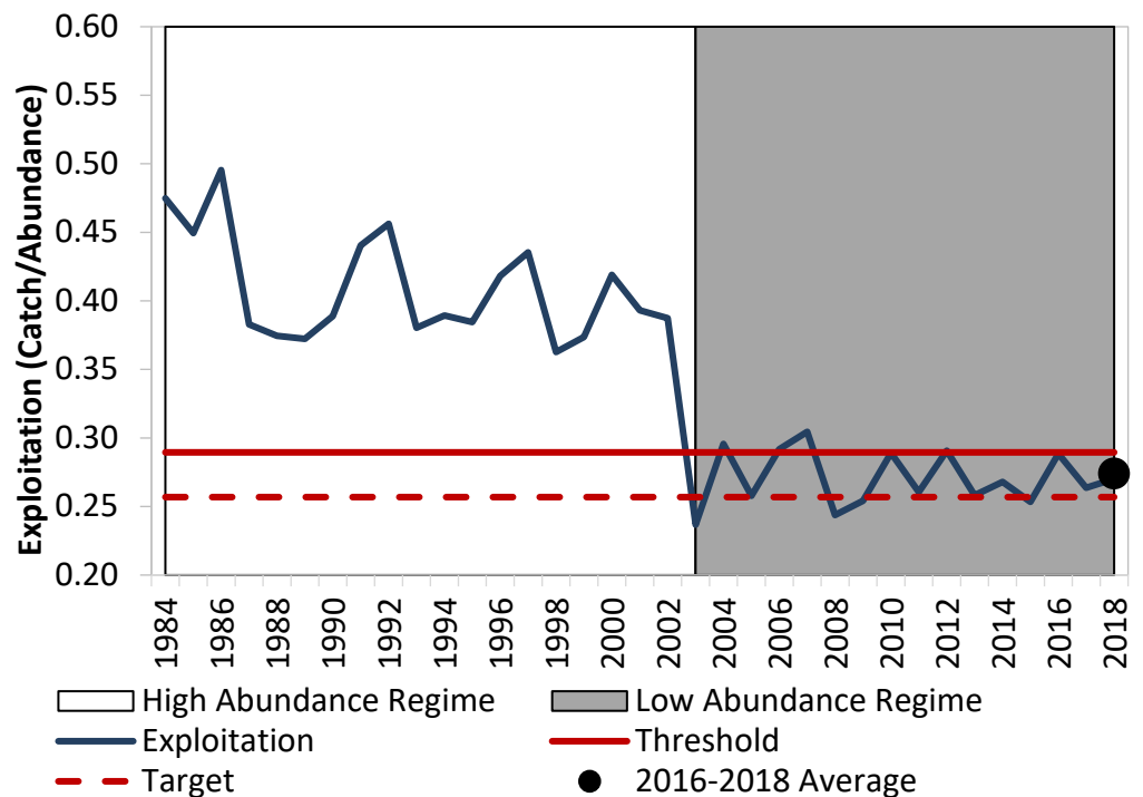
Figure 5. Exploitation for SNE Relative to Reference Points
